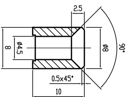
Hole Machining
