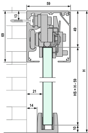
Wandmontage
