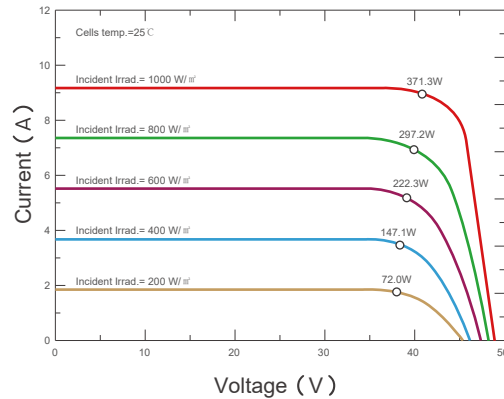
Current-Voltage & Power-Voltage Curves (CP72-6 friline)
