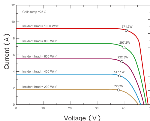
Current-Voltage & Power-Voltage Curves (CP72-4 friline)
