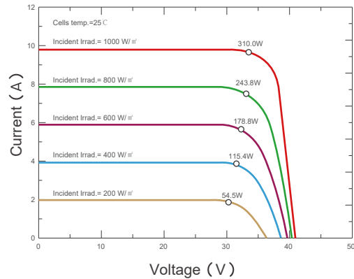
Current-Voltage & Power-Voltage Curves (CP60-4 friline)
