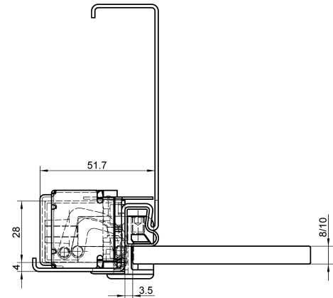
Stahlzarge
