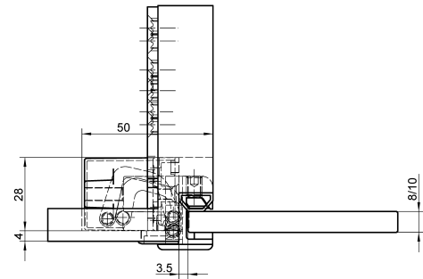
Futterzarge
