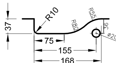
Detail X - DORMA PT 10/20
