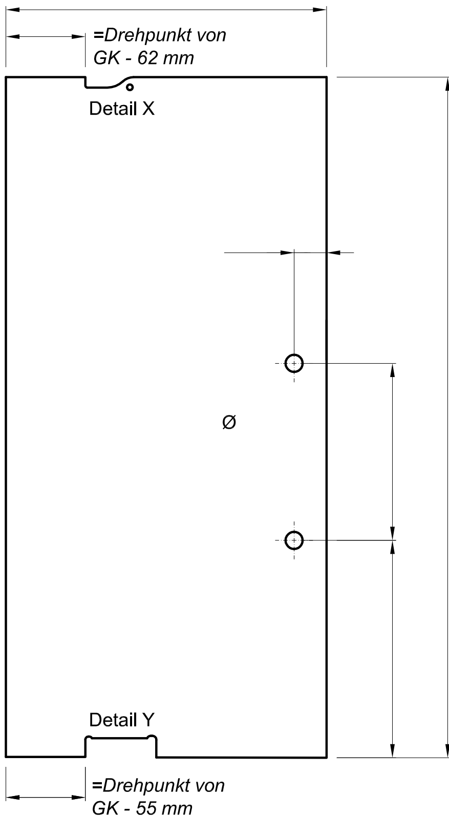
Detail X - DORMA PT 10/20
